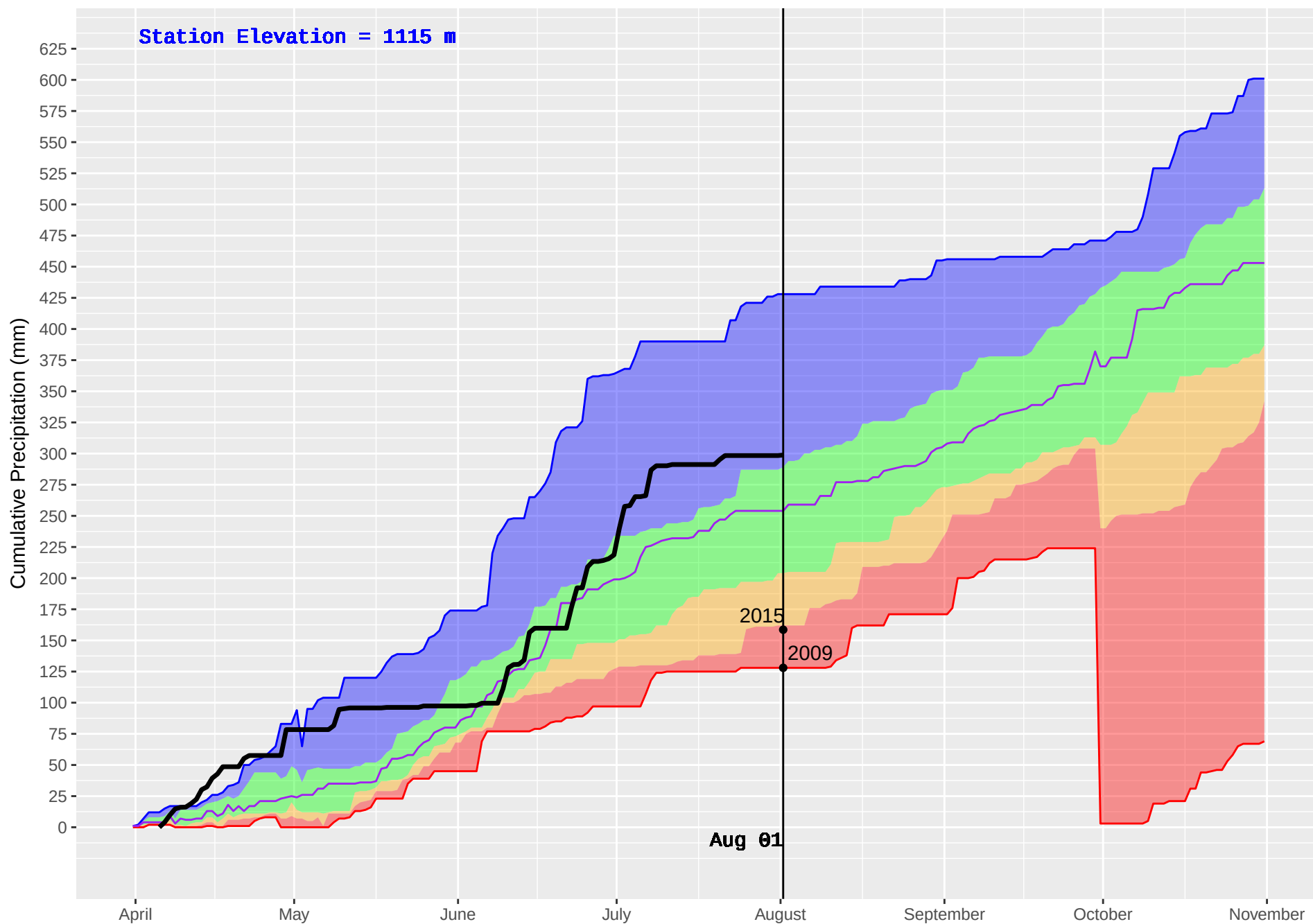
SICAMOUS (882) : Historical (2004–2016) and Current (2018) Daily Cumulative Precipitation
